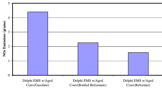
Figure 10. Engine Out NOx Emissions - First Cycle of the FTP Test.
