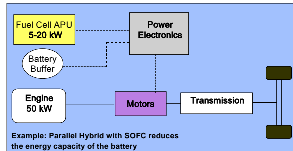
Figure 14. SOFC APU Plus Full Hybrid.
