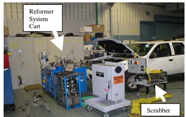
Figure 7. Vehicle and Reformer System Hardware.
