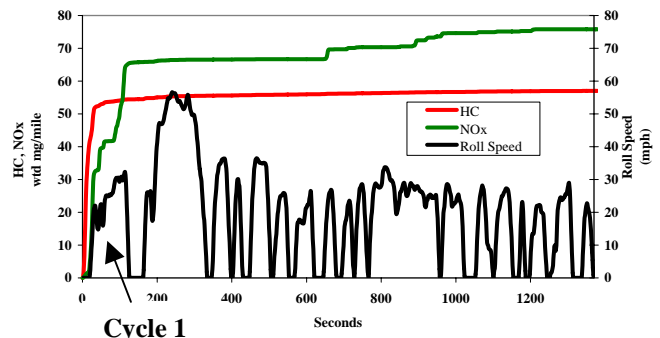
Figure 4. Cumulative HC and NO x Tailpipe Emissions FTP.
