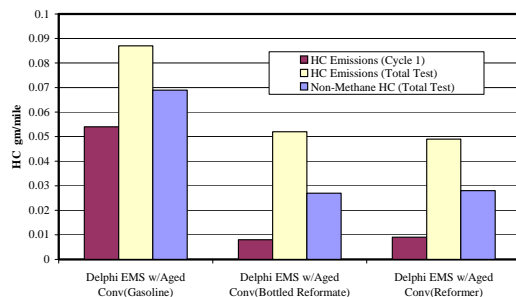
Figure 11. Tailpipe HC Emissions Summary.
