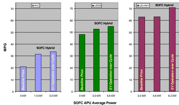
Figure 15. Results of simulation of SOFC hybrids applied to a hybrid vehicle similar to the first generation Toyota Prius.
