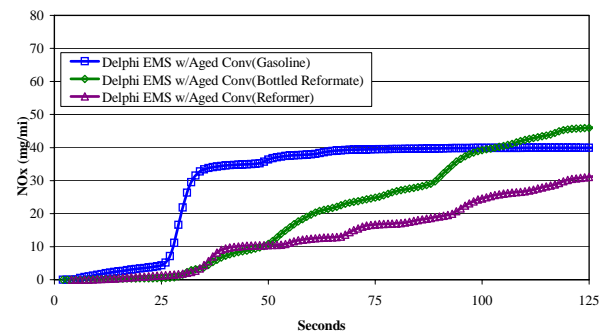
Figure 9. Weighted Tailpipe NOx Emissions - First Cycle of the FTP Test.
