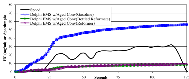
Figure 8. Weighted Tailpipe HC Emissions – First Cycle of the FTP Test
