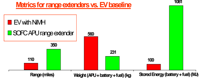
Figure 16. SOFC EV Range Extender Modeling Results
