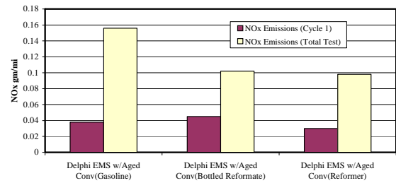
Figure 12. Tailpipe NOx Emissions Summary.
