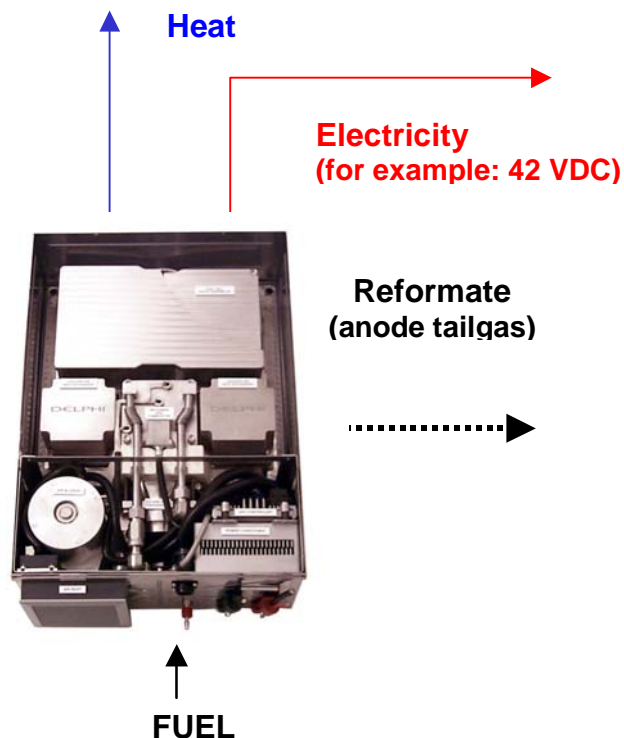
Figure 13. Prototype SOFC APU, showing 3 potential products
