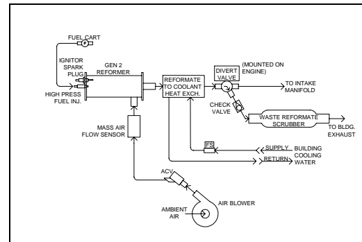
Figure 6. Prototype Gasoline Fuel Reformer and Test Configuration.
