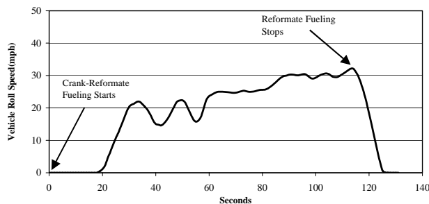
Figure 5. FTP First Cycle Reformate Fueling Strategy.
